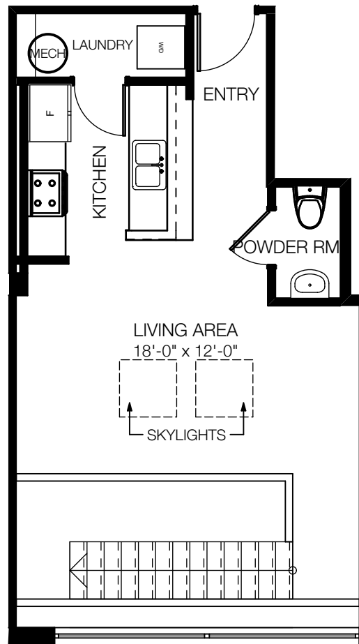
upper level
