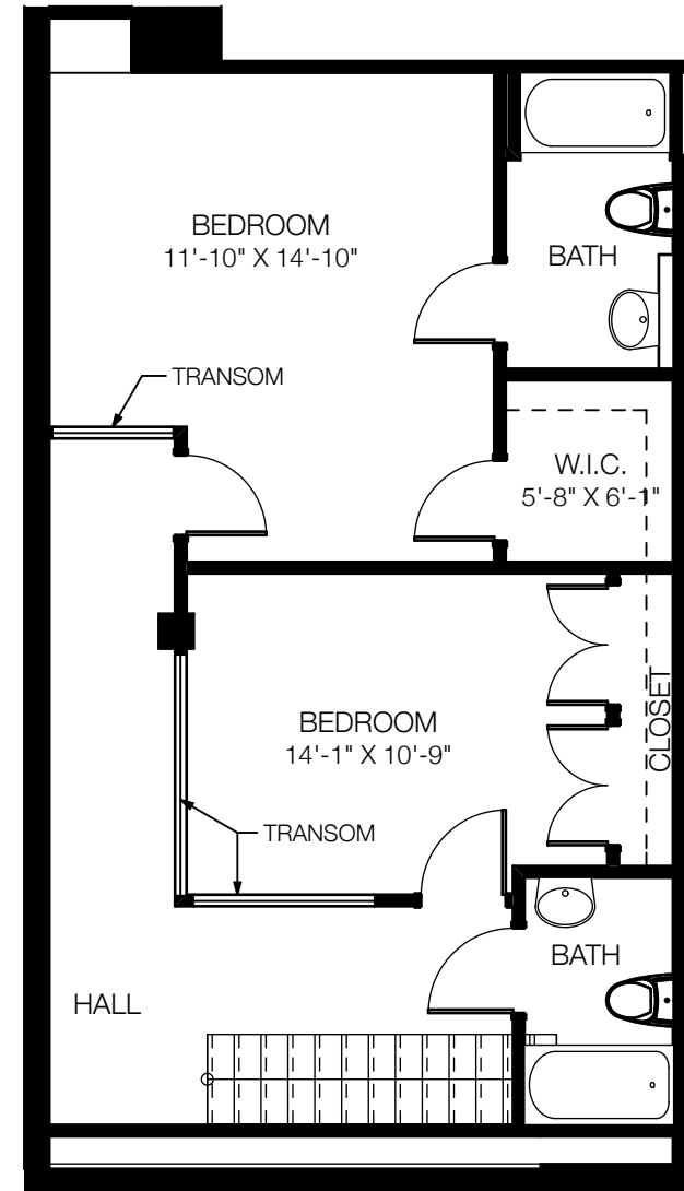
lower level
