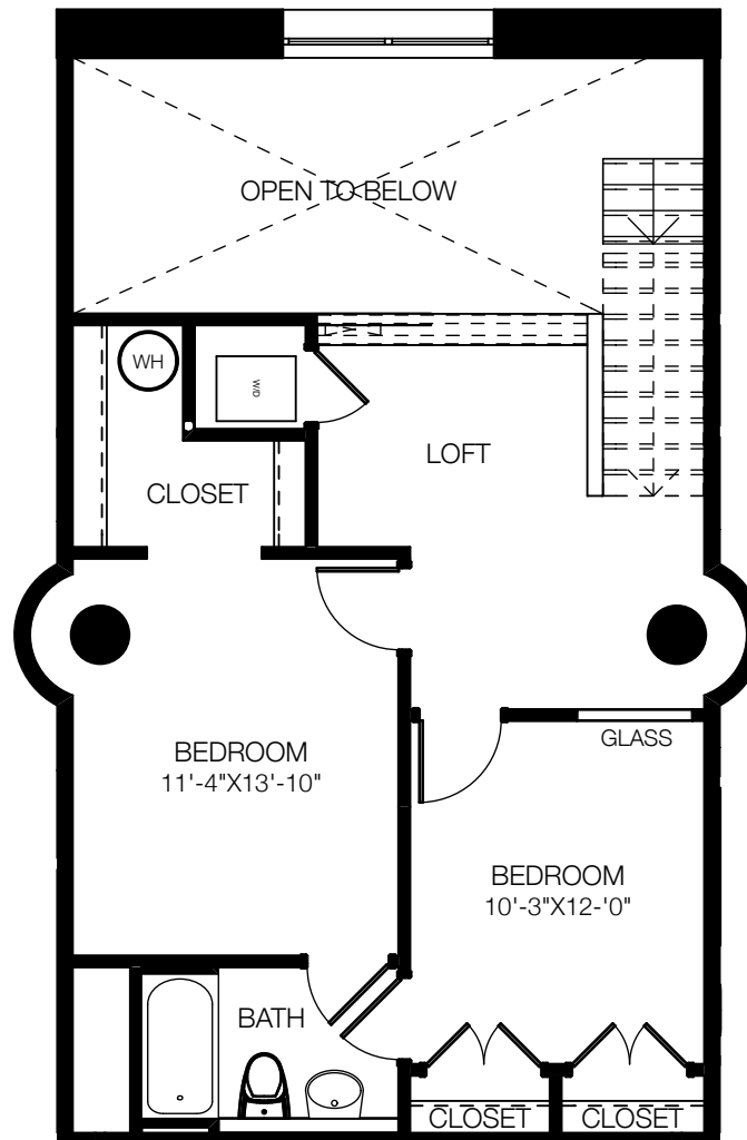
upper level
