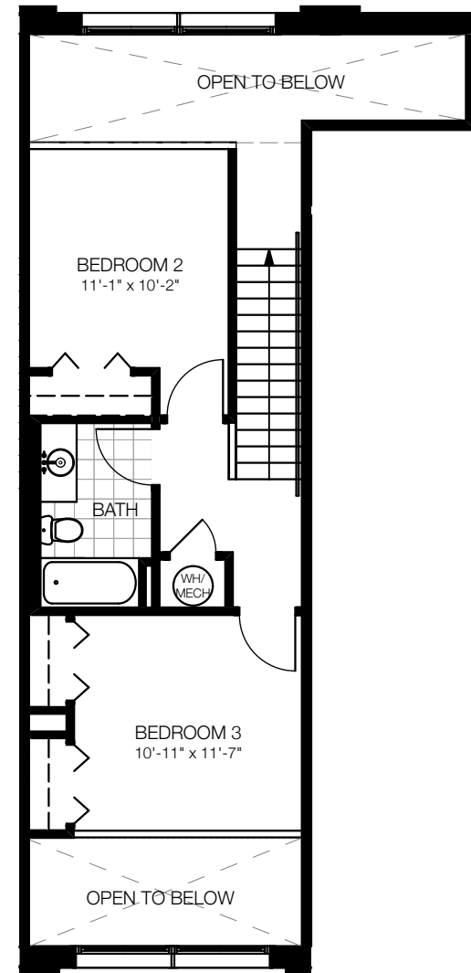
upper floor
